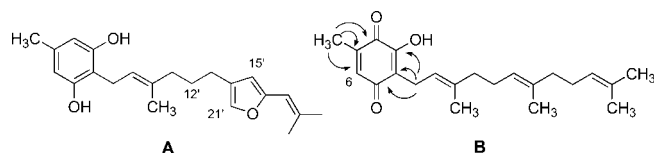
Figure 1. Partial structures A and B for albatrellin (arrows indicate selected couplings from the ^1\text{H} -coupled ^{13}\text{C} NMR spectrum).
