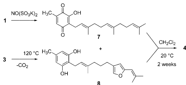
Scheme 1. Synthesis of albatrellin ( 4 ).
